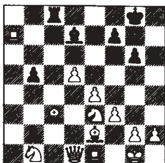
24 Lc3
